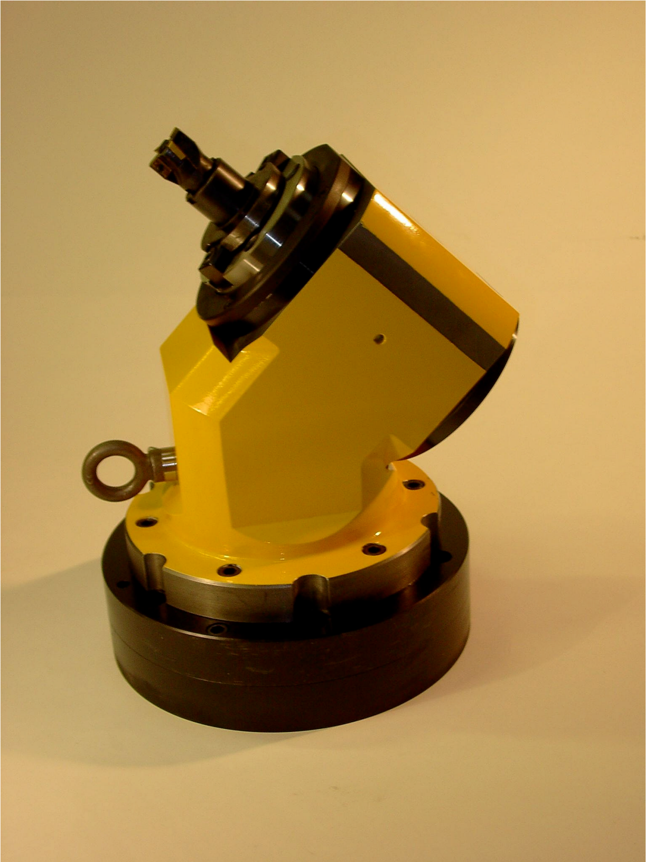
Heavy Duty Fixed Angle Head (45°) Customer - SIEMENS, Newcastle, UK.
